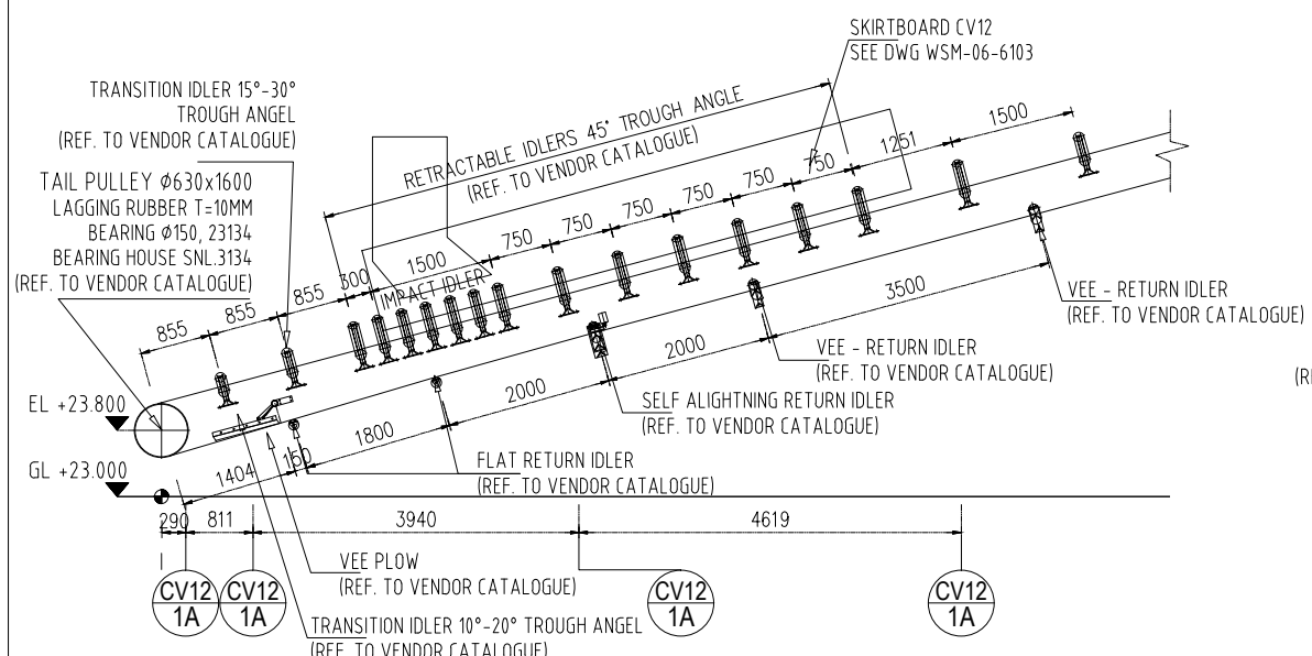
DETAIL 1
