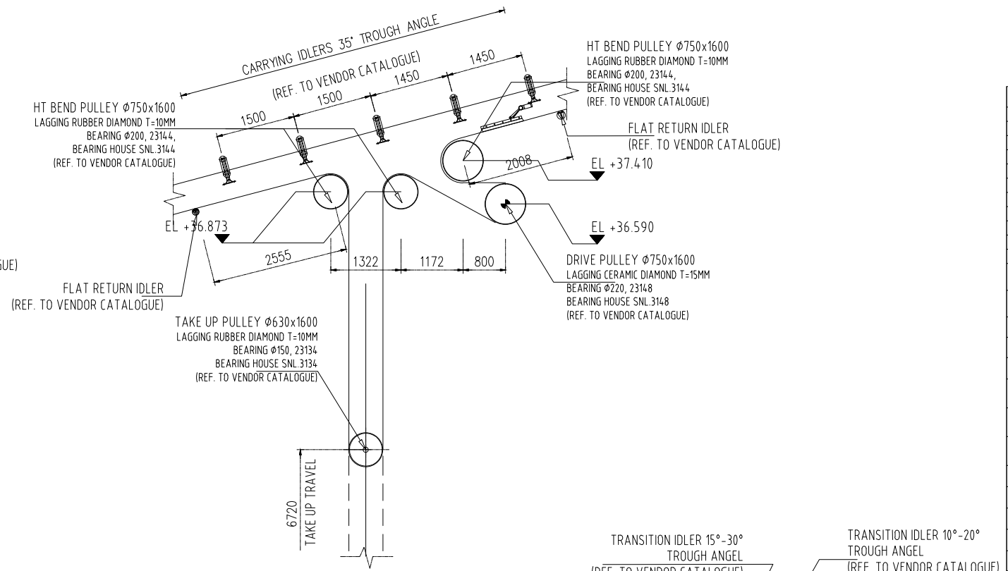
DETAIL 3
